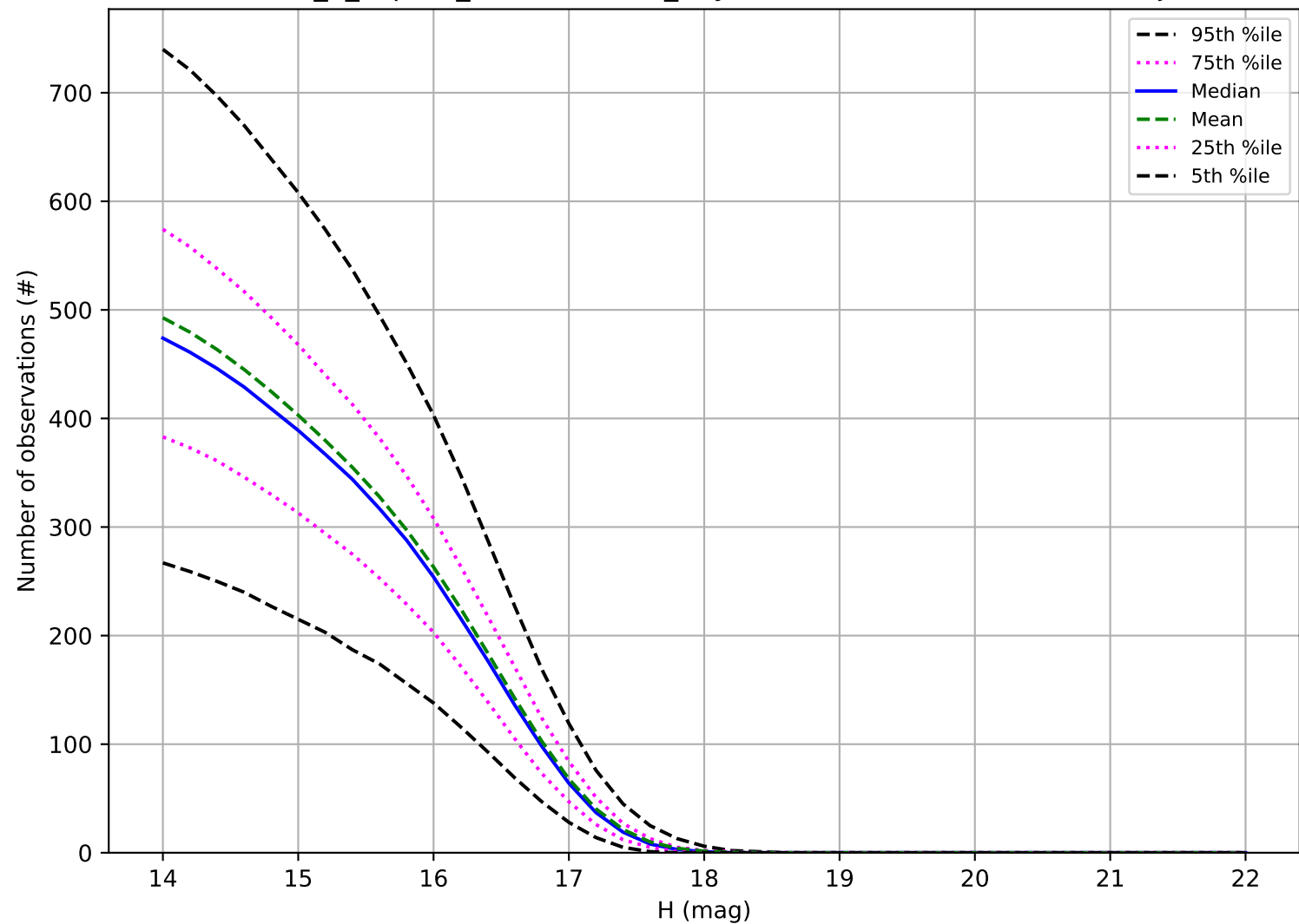
internal_u_expt27_nscale0.9v3.4_10yrs: Number of observations Trojan
