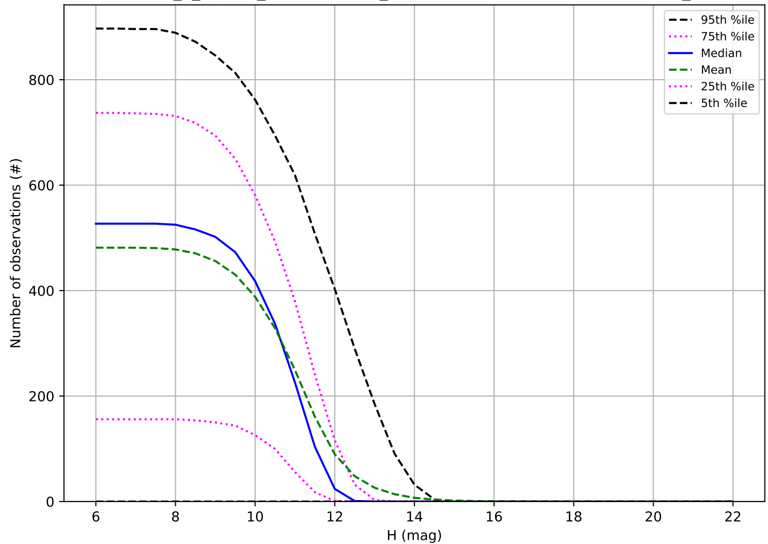
internal_u_expt27_nscale0.9v3.4_10yrs: Number of observations OCC_r20
