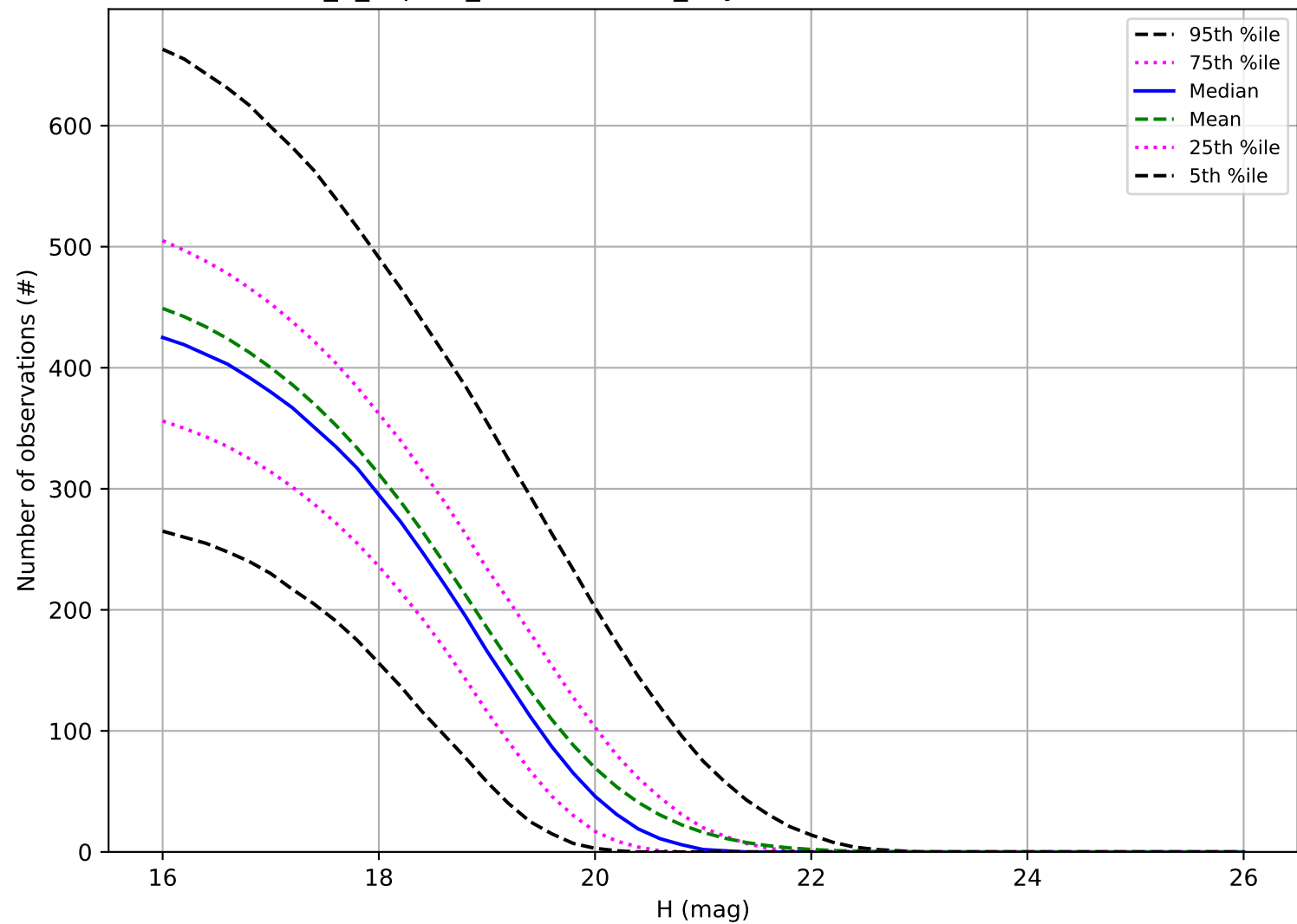
internal_u_expt27_nscale0.9v3.4_10yrs: Number of observations MBA
