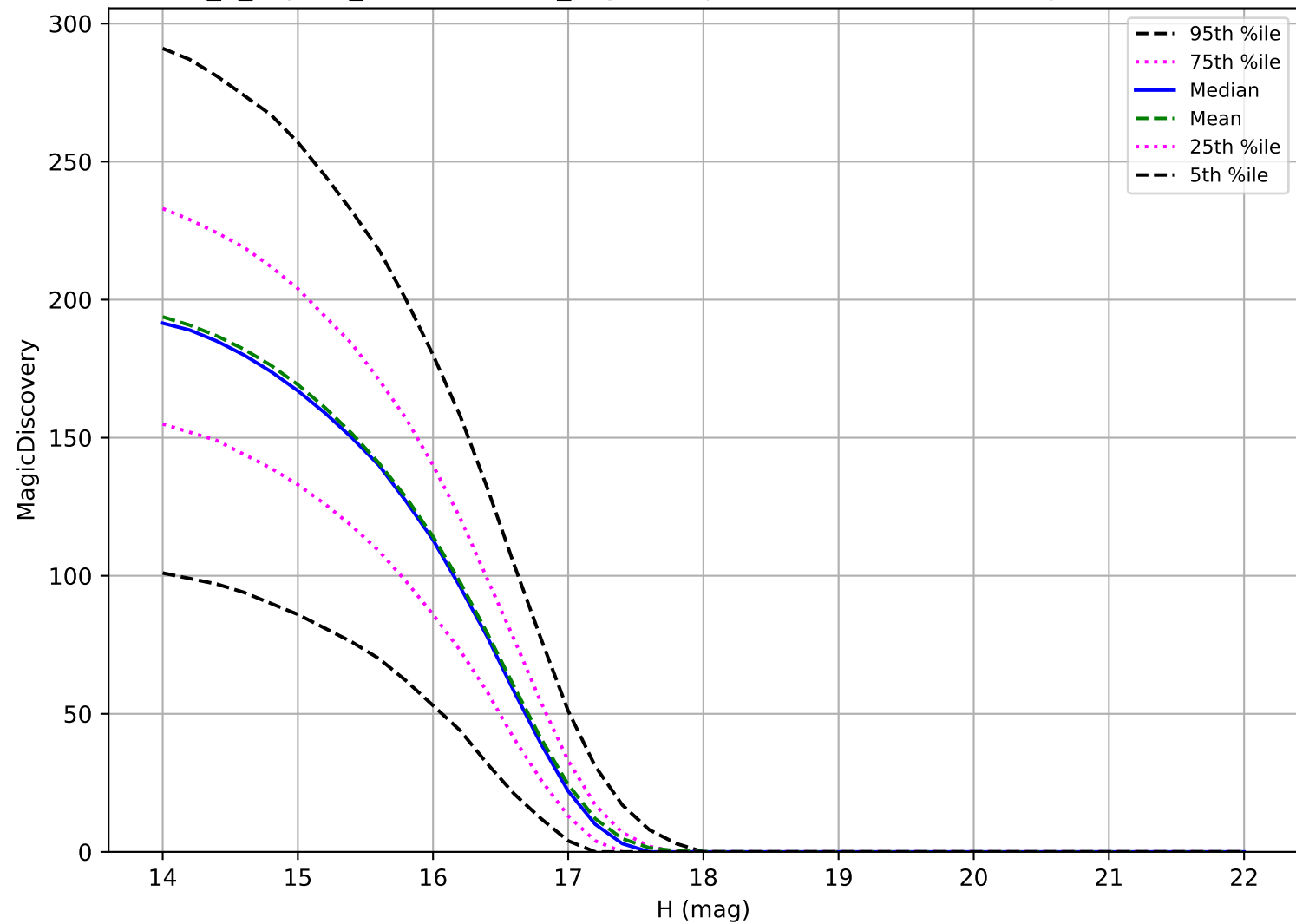
internal_u_expt27_nscale0.9v3.4_10yrs: Trojan 6 detections in 60 nights detection loss
