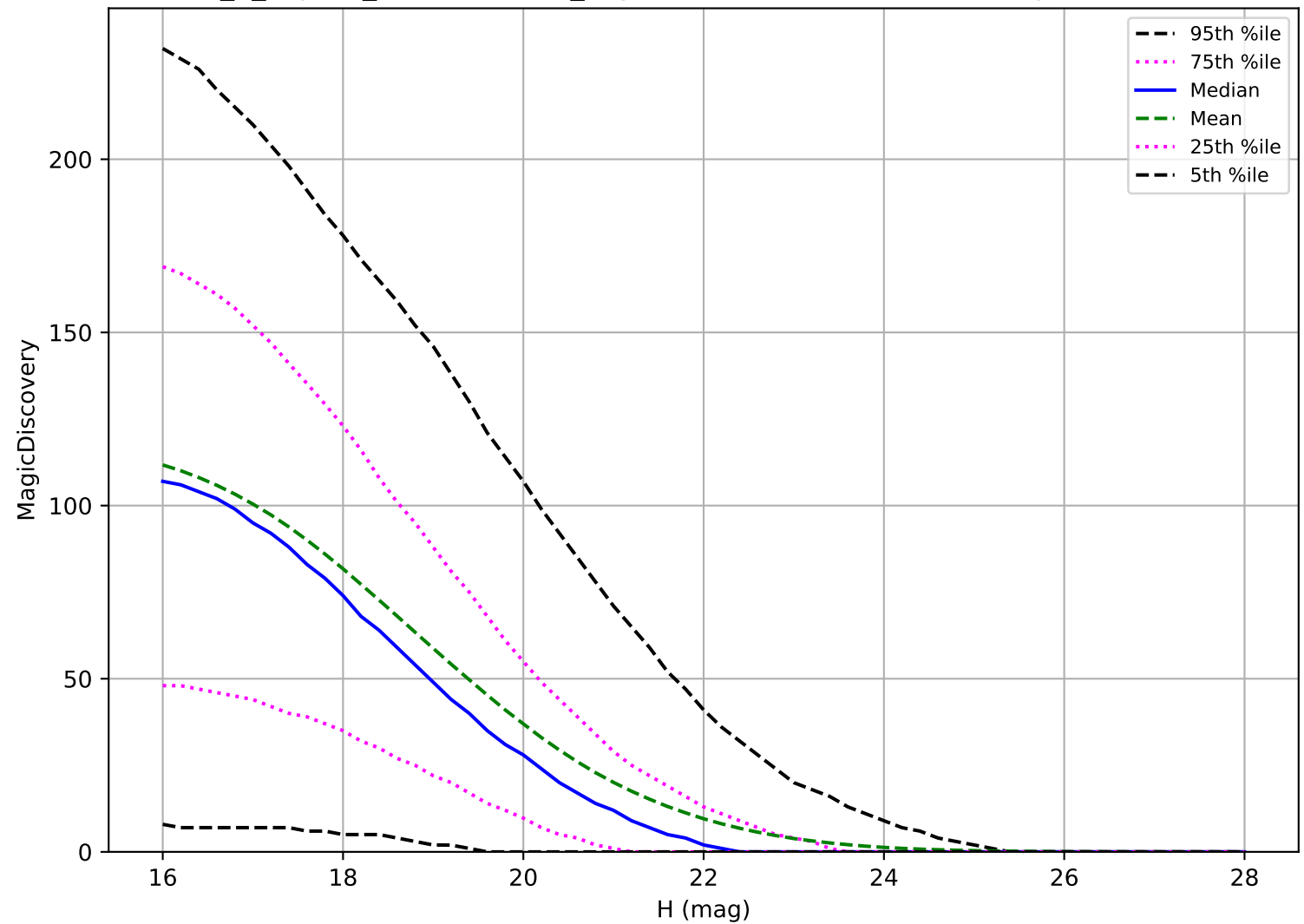
internal_u_expt27_nscale0.9v3.4_10yrs: PHA 6 detections in 60 nights detection loss
