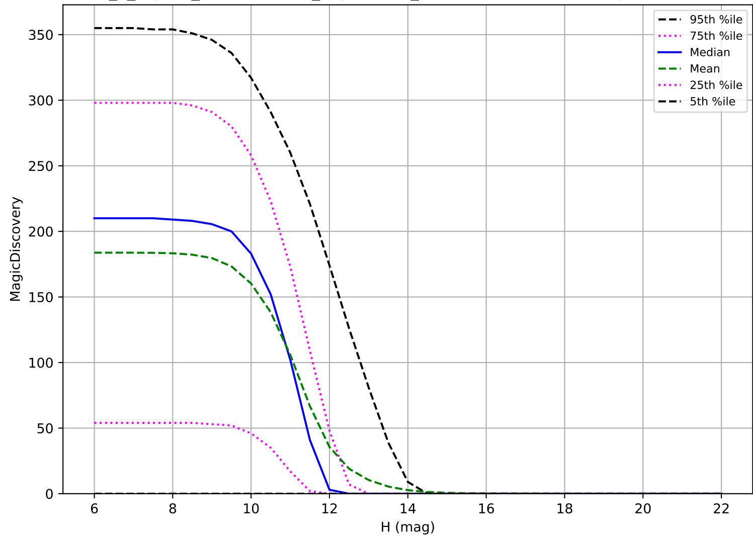
internal_u_expt27_nscale0.9v3.4_10yrs: OCC_r20 6 detections in 60 nights detection loss
