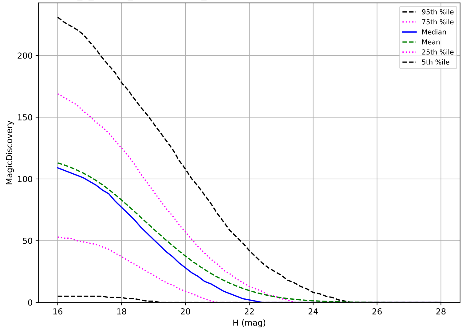
internal_u_expt27_nscale0.9v3.4_10yrs: NEO 6 detections in 60 nights detection loss
