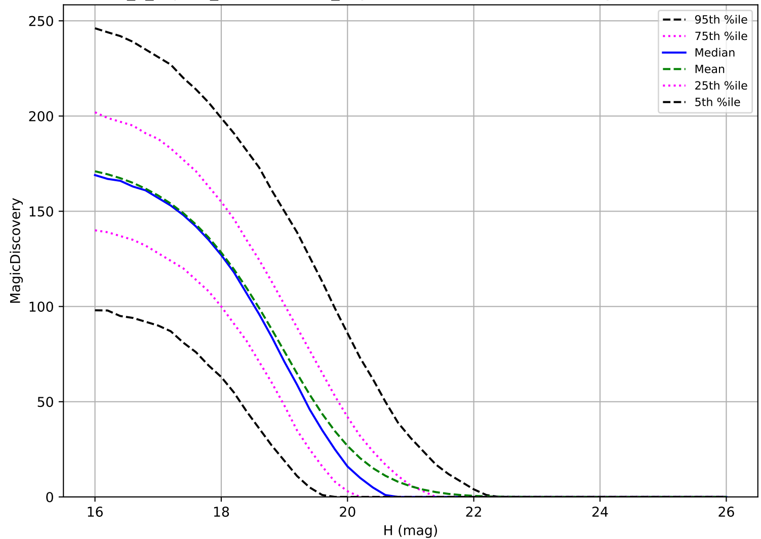
internal_u_expt27_nscale0.9v3.4_10yrs: MBA 6 detections in 60 nights detection loss
