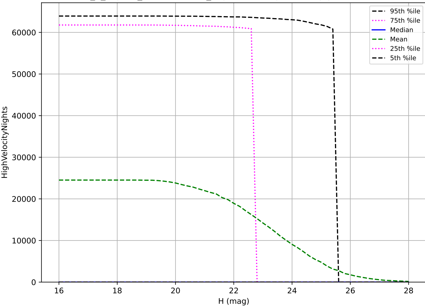
internal_u_expt27_nscale0.9v3.4_10yrs: PHA High velocity pair detection loss
