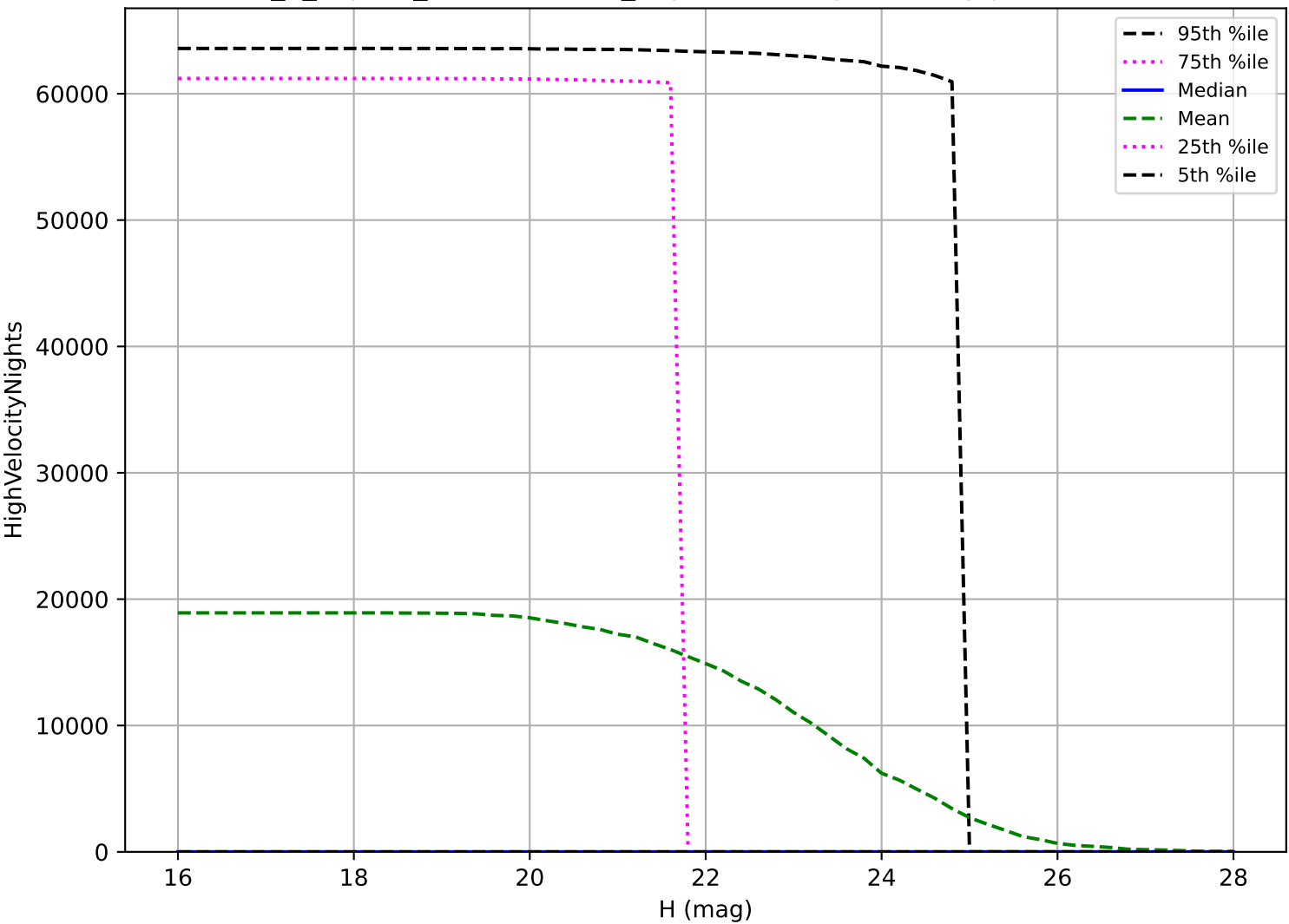
internal_u_expt27_nscale0.9v3.4_10yrs: NEO High velocity pair detection loss
