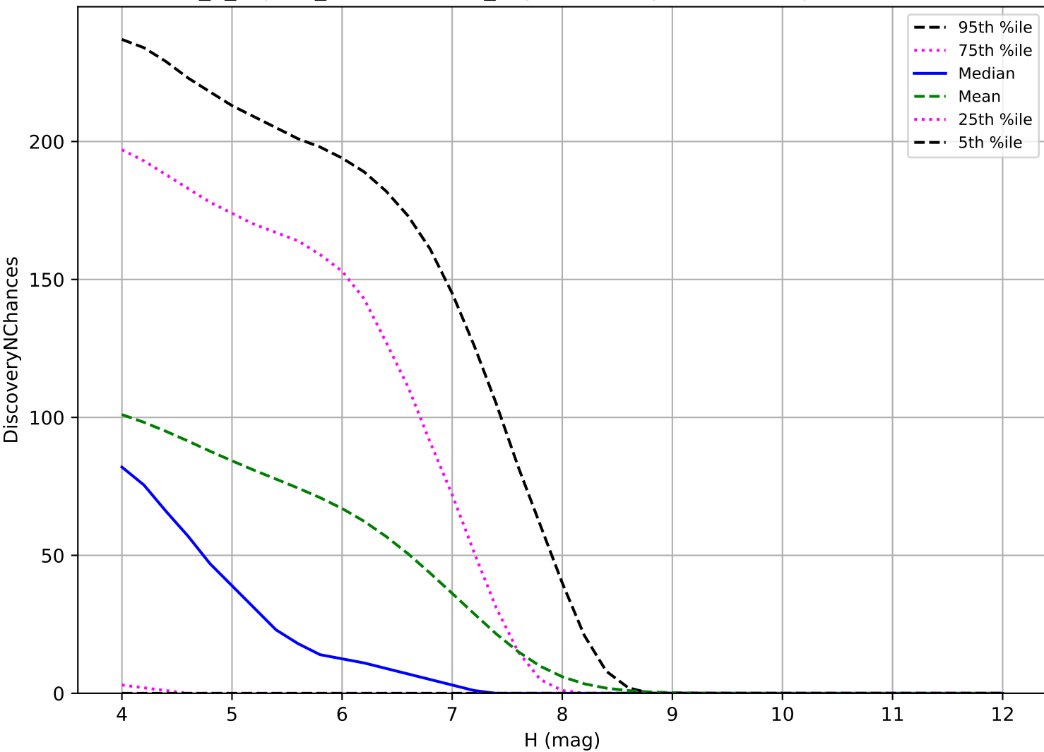
internal_u_expt27_nscale0.9v3.4_10yrs: TNO 3 pairs in 15 nights detection loss
