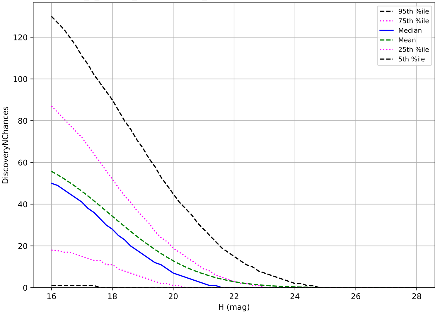
internal_u_expt27_nscale0.9v3.4_10yrs: PHA 3 pairs in 15 nights detection loss
