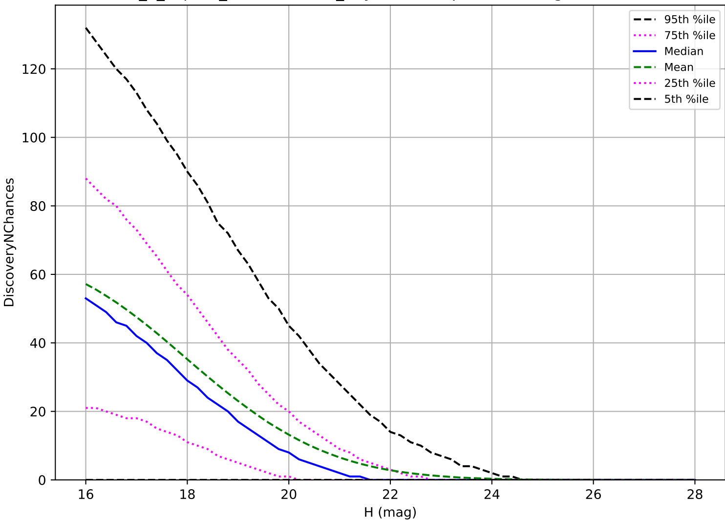
internal_u_expt27_nscale0.9v3.4_10yrs: NEO 3 pairs in 15 nights detection loss
