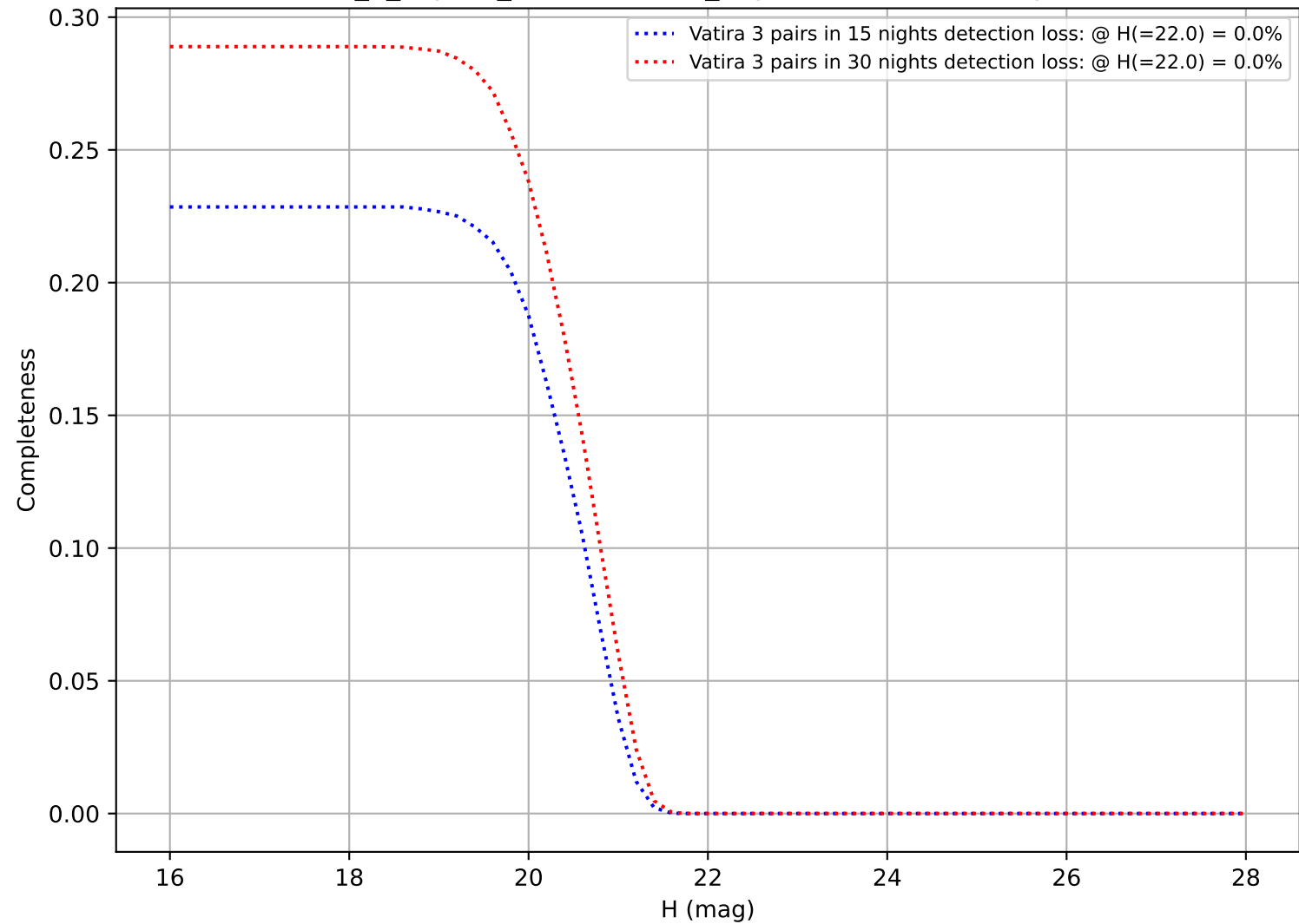
internal_u_expt27_nscale0.9v3.4_10yrs: DifferentialCompleteness
