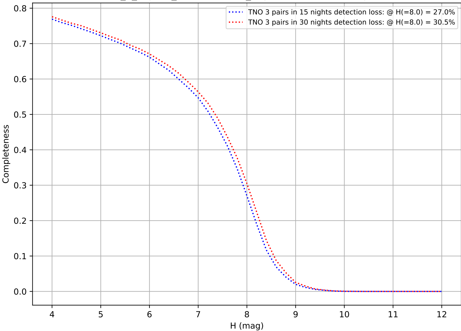
internal_u_expt27_nscale0.9v3.4_10yrs: DifferentialCompleteness
