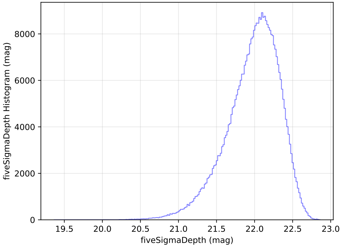
internal_u_expt27_nscale0.9v3.4_10yrs y: fiveSigmaDepth Histogram
