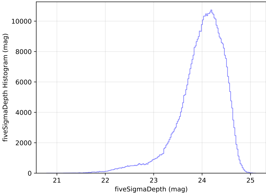
internal_u_expt27_nscale0.9v3.4_10yrs r: fiveSigmaDepth Histogram
