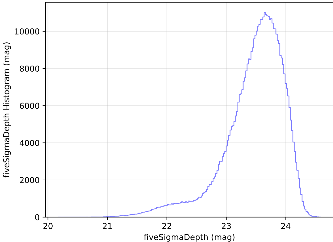
internal_u_expt27_nscale0.9v3.4_10yrs i: fiveSigmaDepth Histogram
