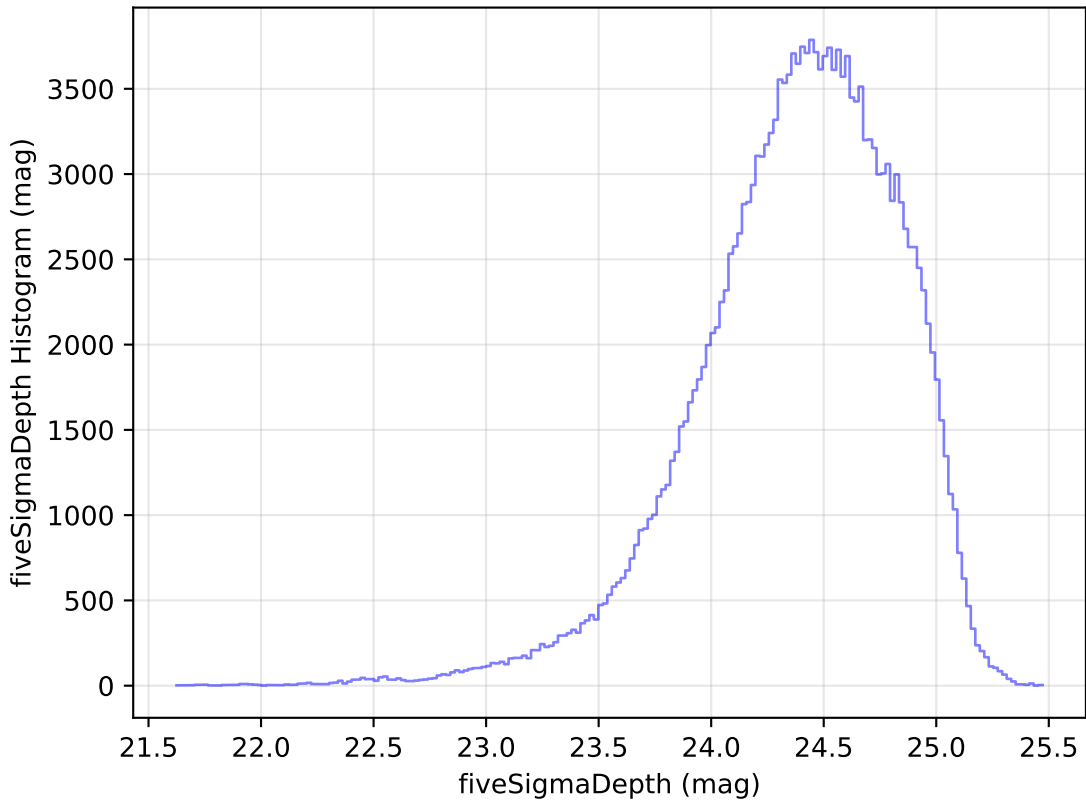
internal_u_expt27_nscale0.9v3.4_10yrs g: fiveSigmaDepth Histogram
