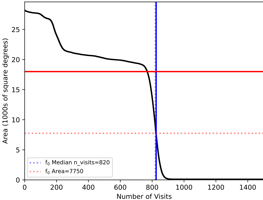
internal_u_expt27_nscale0.9v3.4_10yrs : fO
