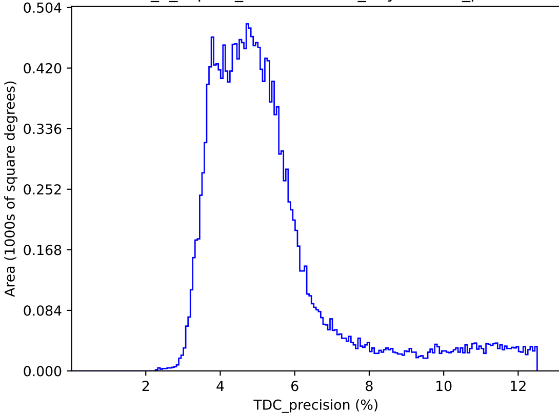
internal_u_expt27_nscale0.9v3.4_10yrs : TDC_precision
