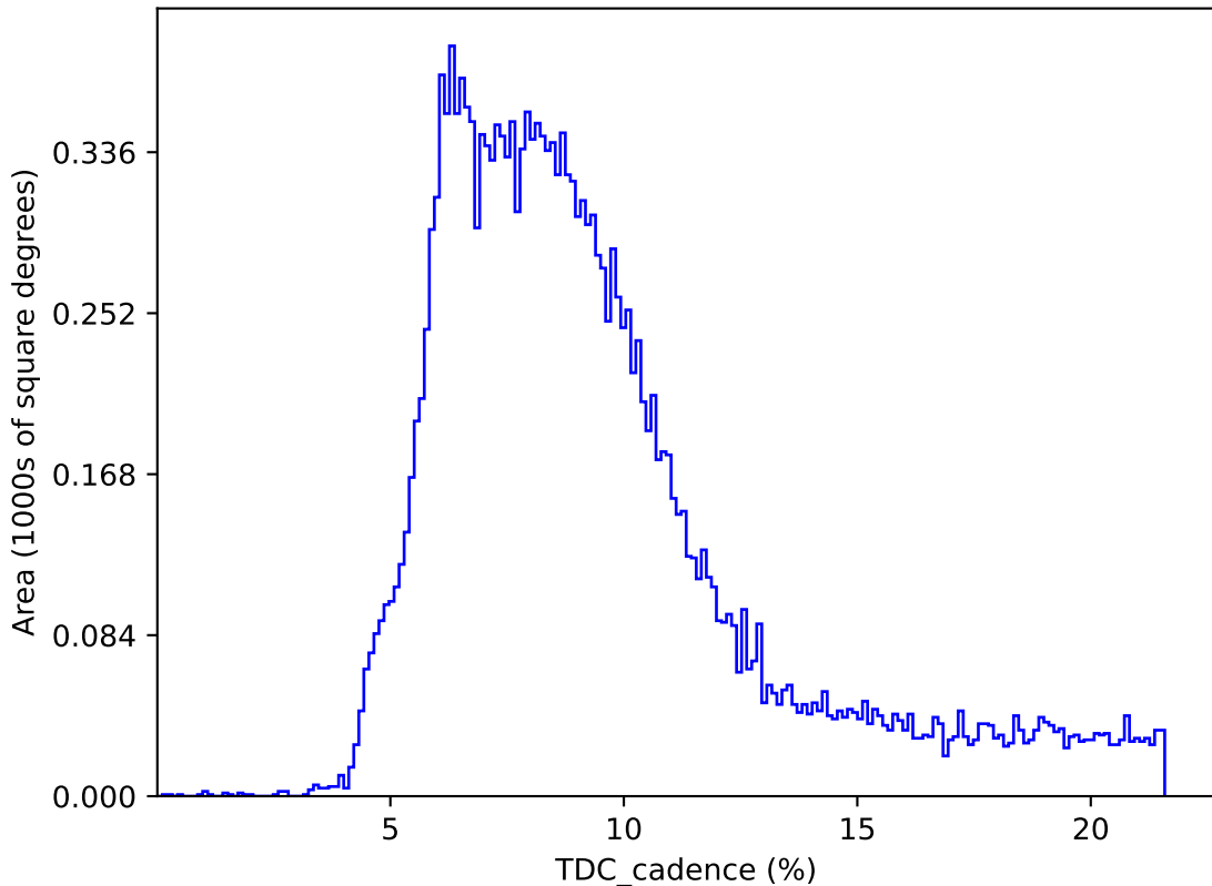
internal_u_expt27_nscale0.9v3.4_10yrs : TDC_cadence
