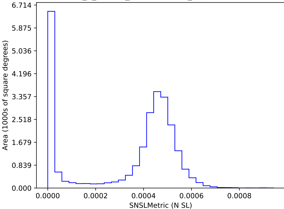
internal_u_expt27_nscale0.9v3.4_10yrs : SNSLMetric
