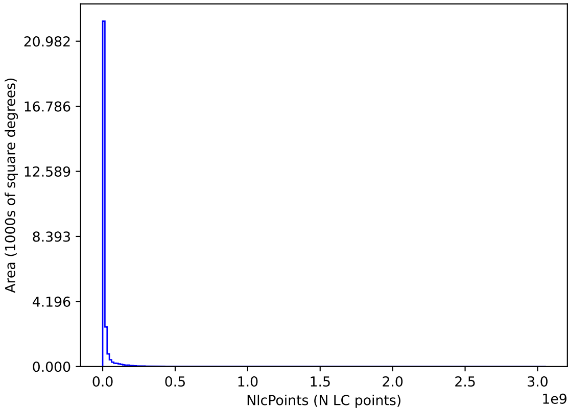
internal_u_expt27_nscale0.9v3.4_10yrs : NlcPoints
