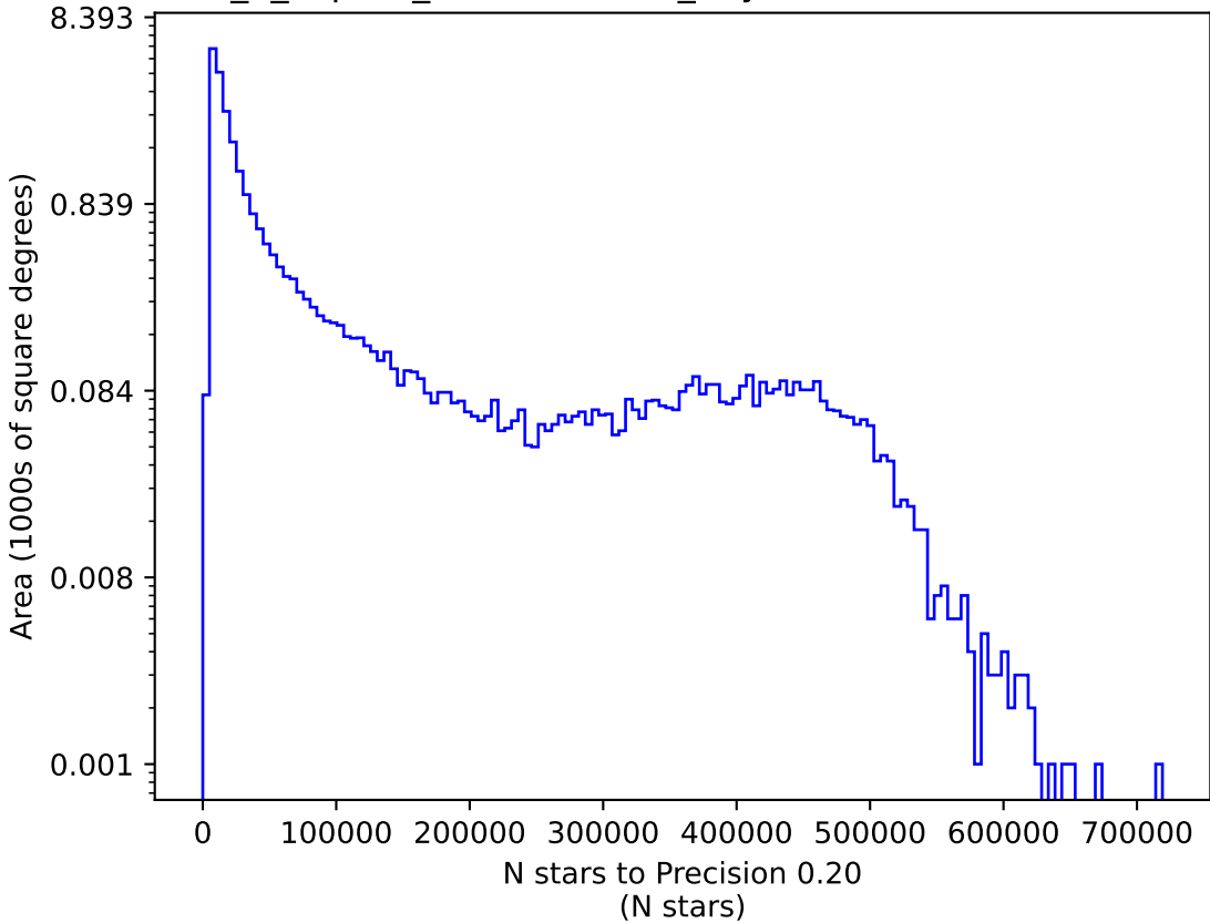
internal_u_expt27_nscale0.9v3.4_10yrs i: N stars to Precision 0.20
