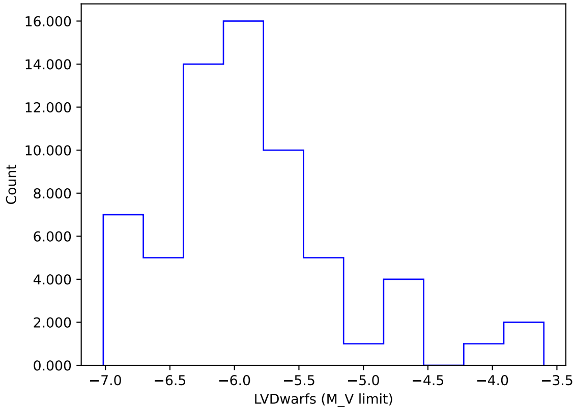
internal_u_expt27_nscale0.9v3.4_10yrs gi: LVDwarfs
