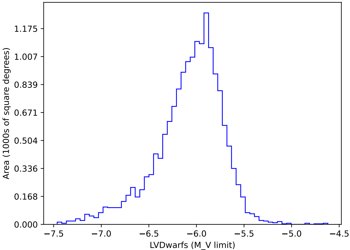
internal_u_expt27_nscale0.9v3.4_10yrs gi: LVDwarfs
