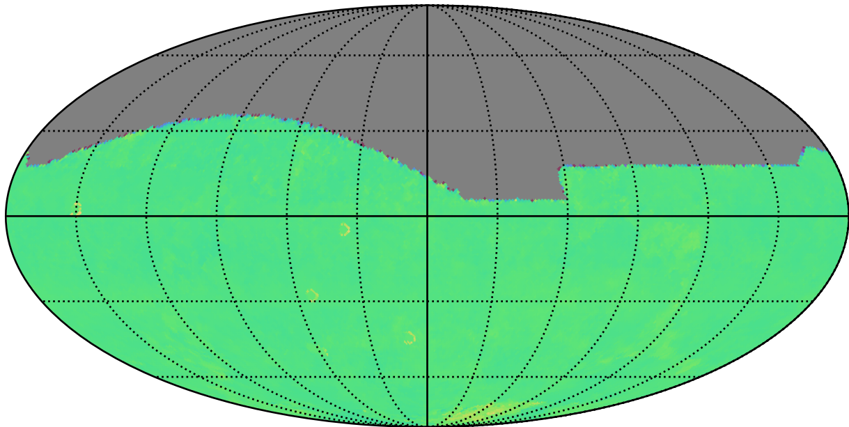
internal_u_expt27_nscale0.9v3.4_10yrs r: Kuiper rotTelPos
