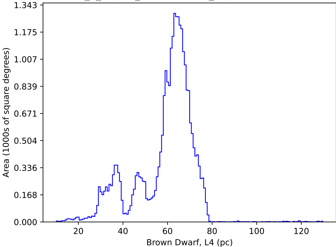
internal_u_expt27_nscale0.9v3.4_10yrs : Brown Dwarf, L4
