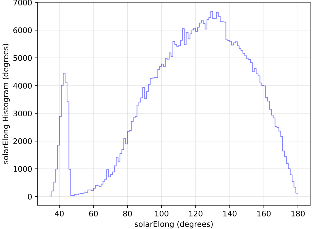
internal_u_expt27_nscale0.9v3.4_10yrs WFD z band: solarElong Histogram
