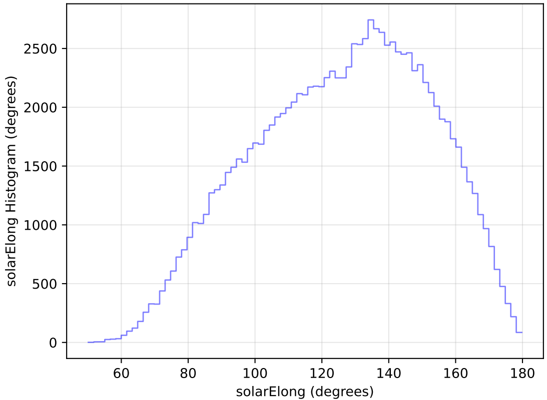
internal_u_expt27_nscale0.9v3.4_10yrs WFD u band: solarElong Histogram
