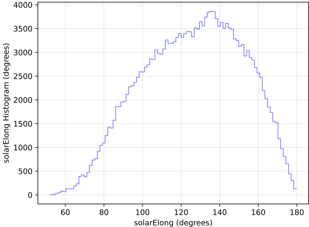
internal_u_expt27_nscale0.9v3.4_10yrs WFD g band: solarElong Histogram
