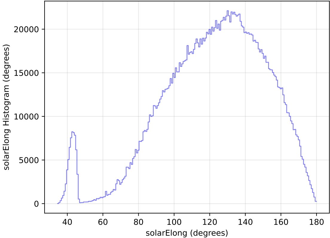
internal_u_expt27_nscale0.9v3.4_10yrs WFD all bands: solarElong Histogram
