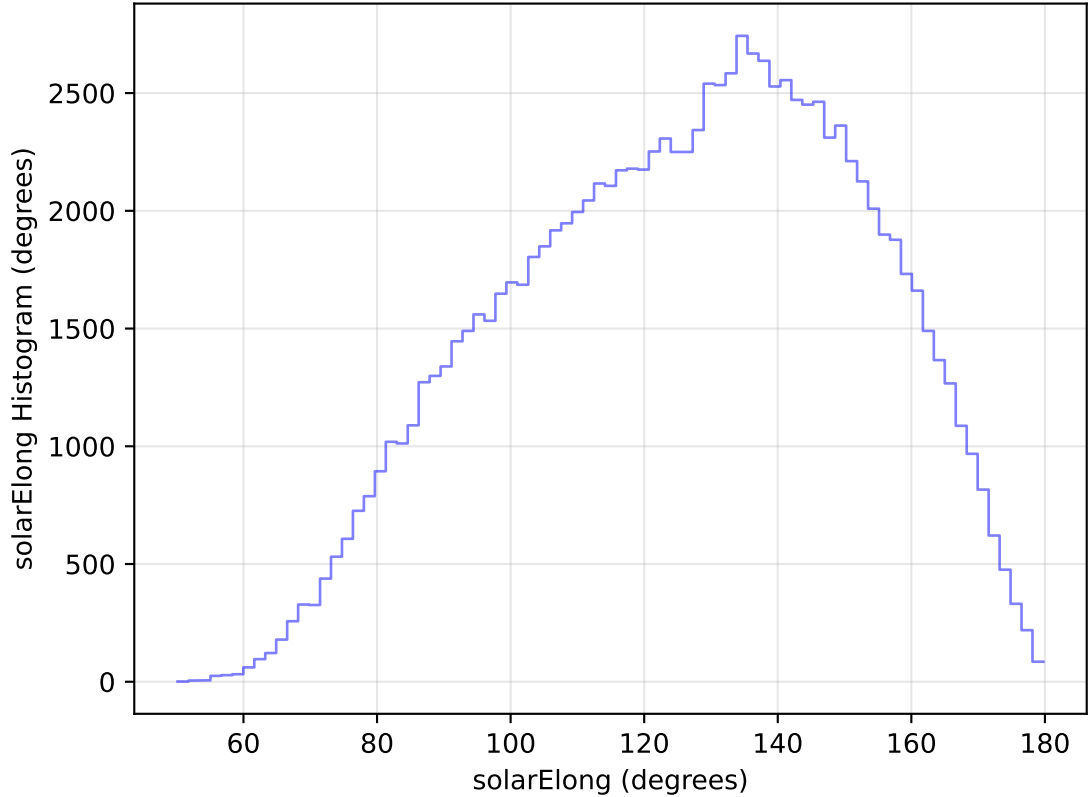
internal_u_expt27_nscale0.9v3.4_10yrs All sky u band: solarElong Histogram
