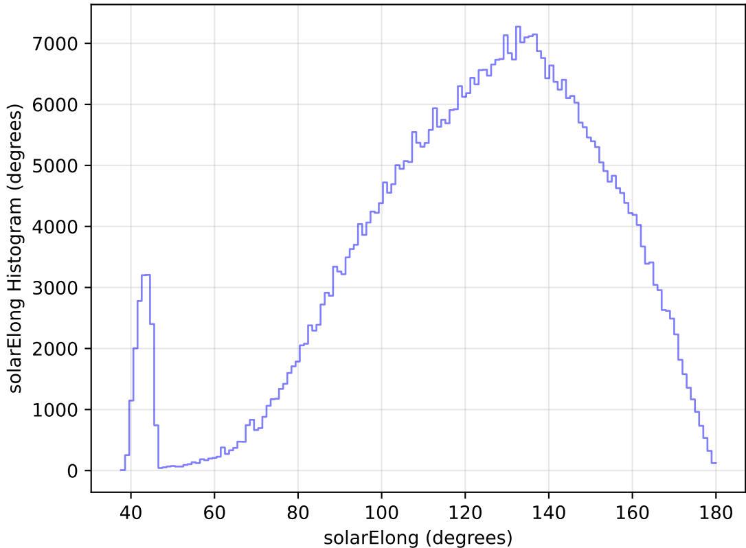
internal_u_expt27_nscale0.9v3.4_10yrs All sky r band: solarElong Histogram
