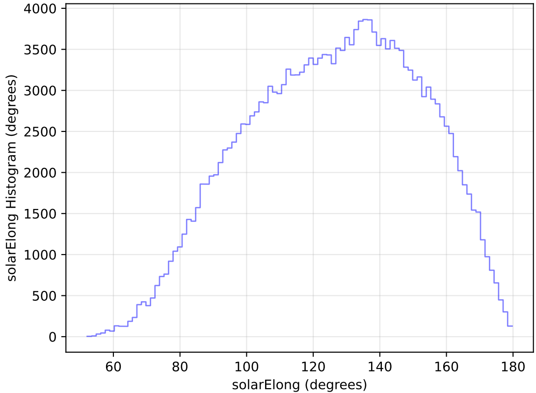
internal_u_expt27_nscale0.9v3.4_10yrs All sky g band: solarElong Histogram
