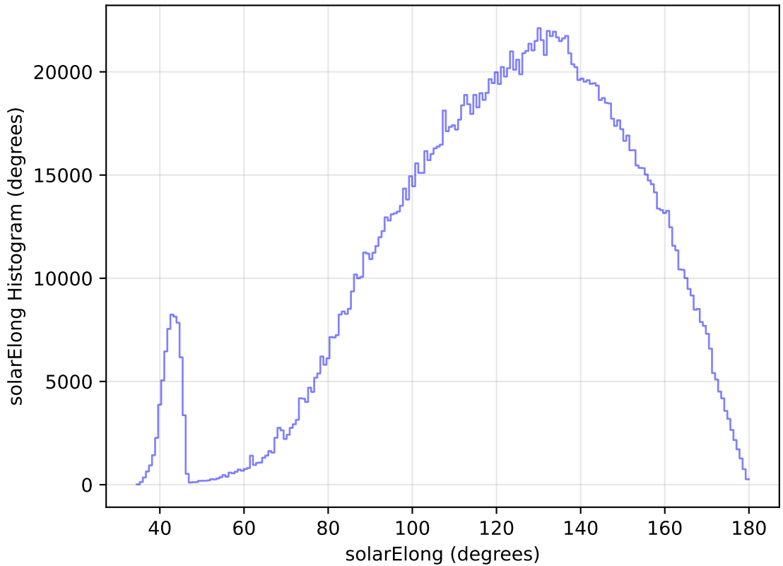
internal_u_expt27_nscale0.9v3.4_10yrs All sky all bands: solarElong Histogram
