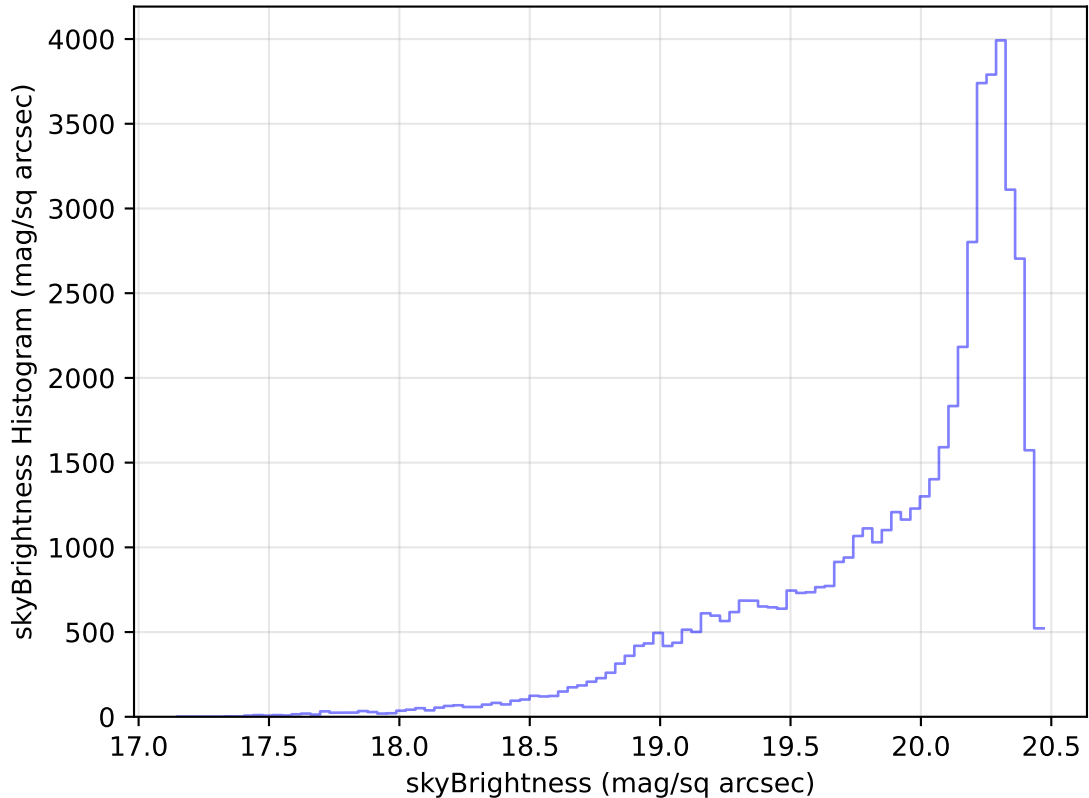
internal_u_expt27_nscale0.9v3.4_10yrs Yr 1 i band: skyBrightness Histogram
