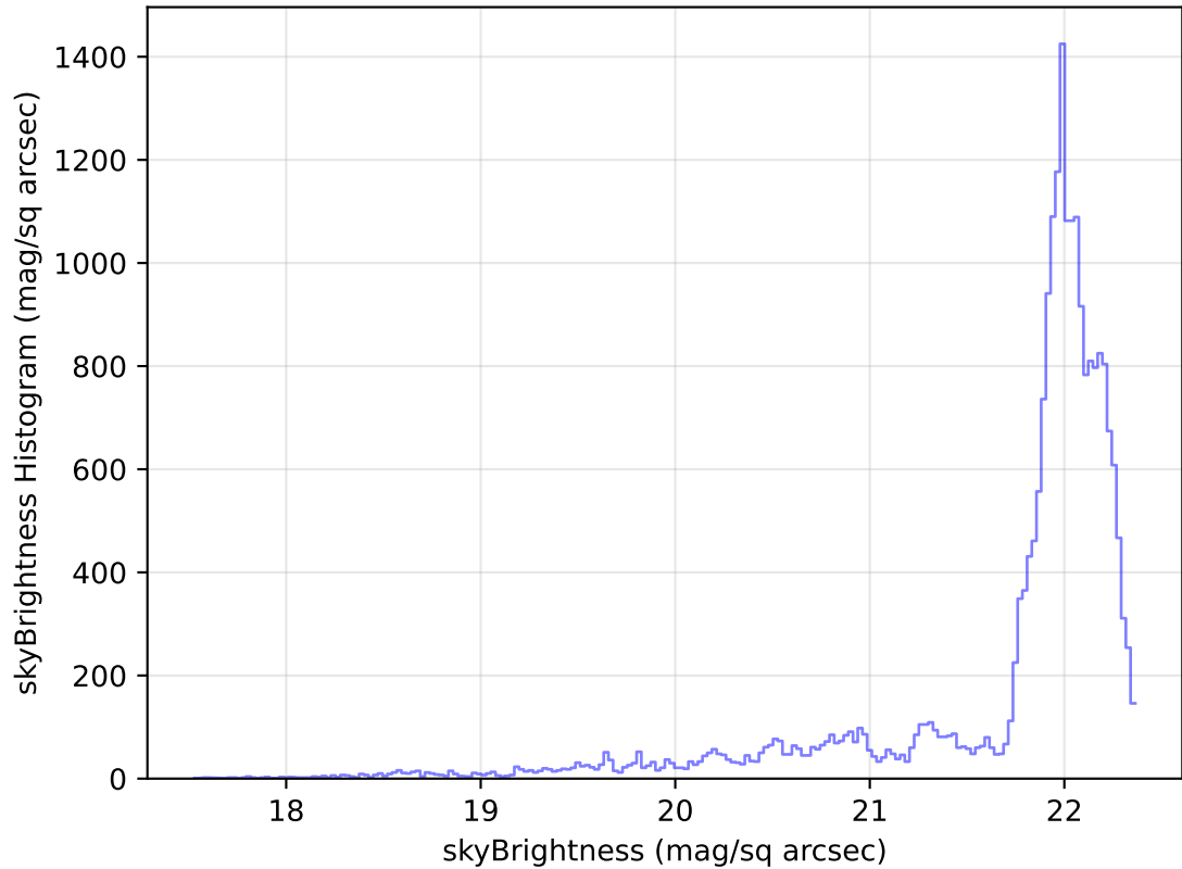
internal_u_expt27_nscale0.9v3.4_10yrs Yr 1 g band: skyBrightness Histogram
