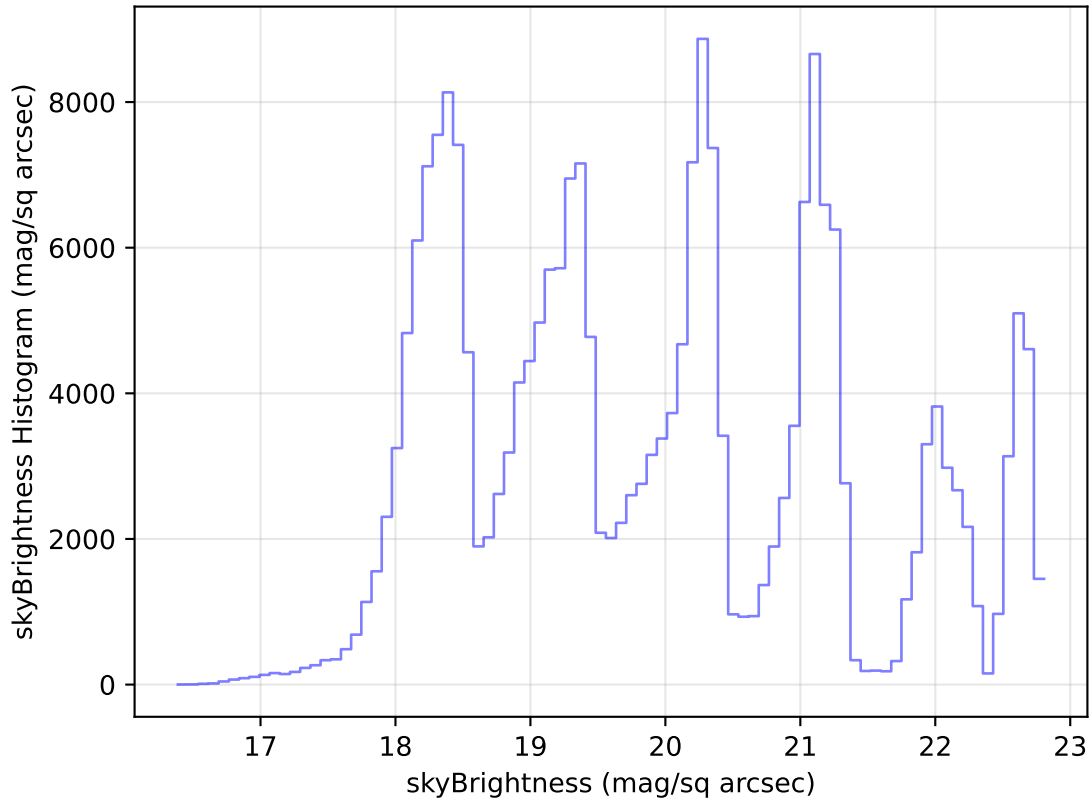
internal_u_expt27_nscale0.9v3.4_10yrs Yr 1 all bands: skyBrightness Histogram
