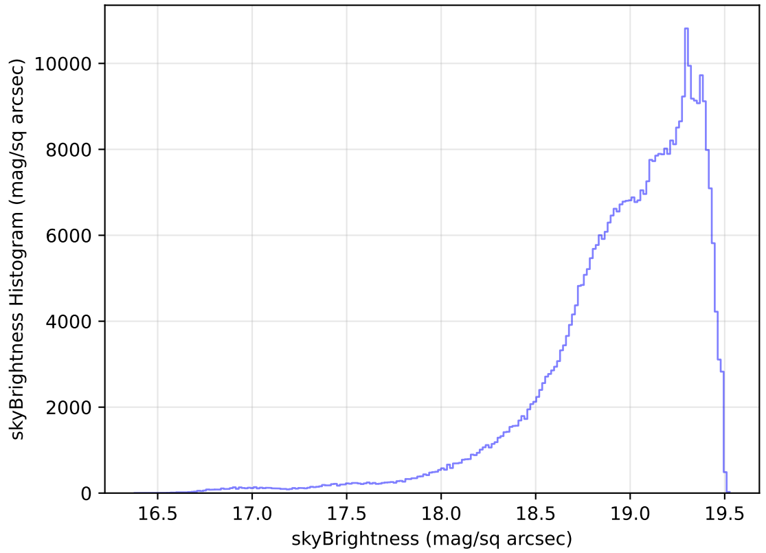
internal_u_expt27_nscale0.9v3.4_10yrs WFD z band: skyBrightness Histogram
