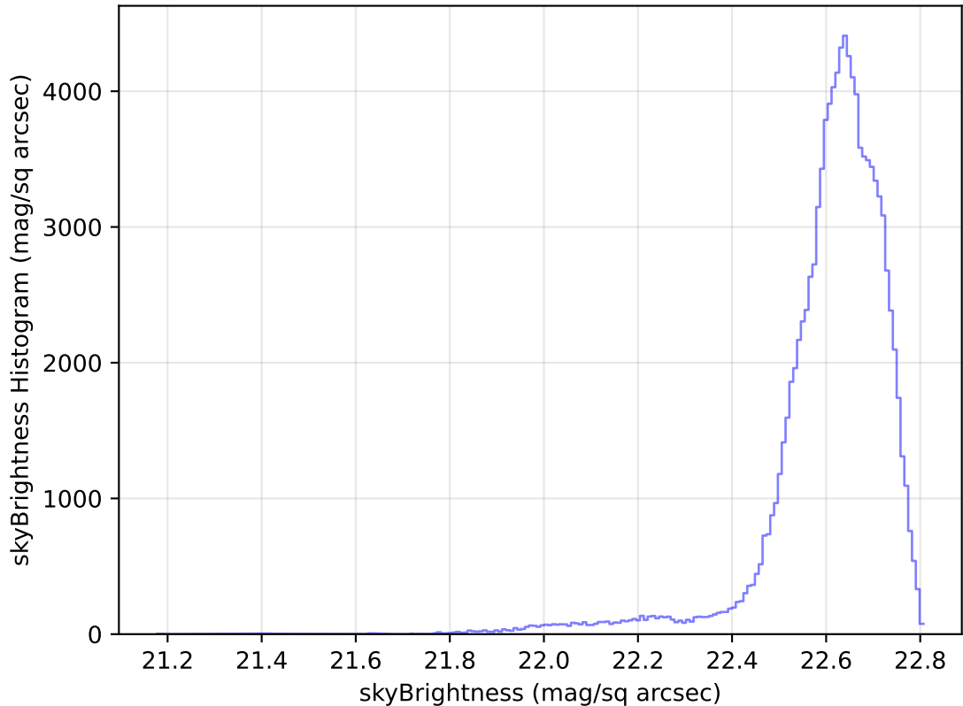
internal_u_expt27_nscale0.9v3.4_10yrs WFD u band: skyBrightness Histogram
