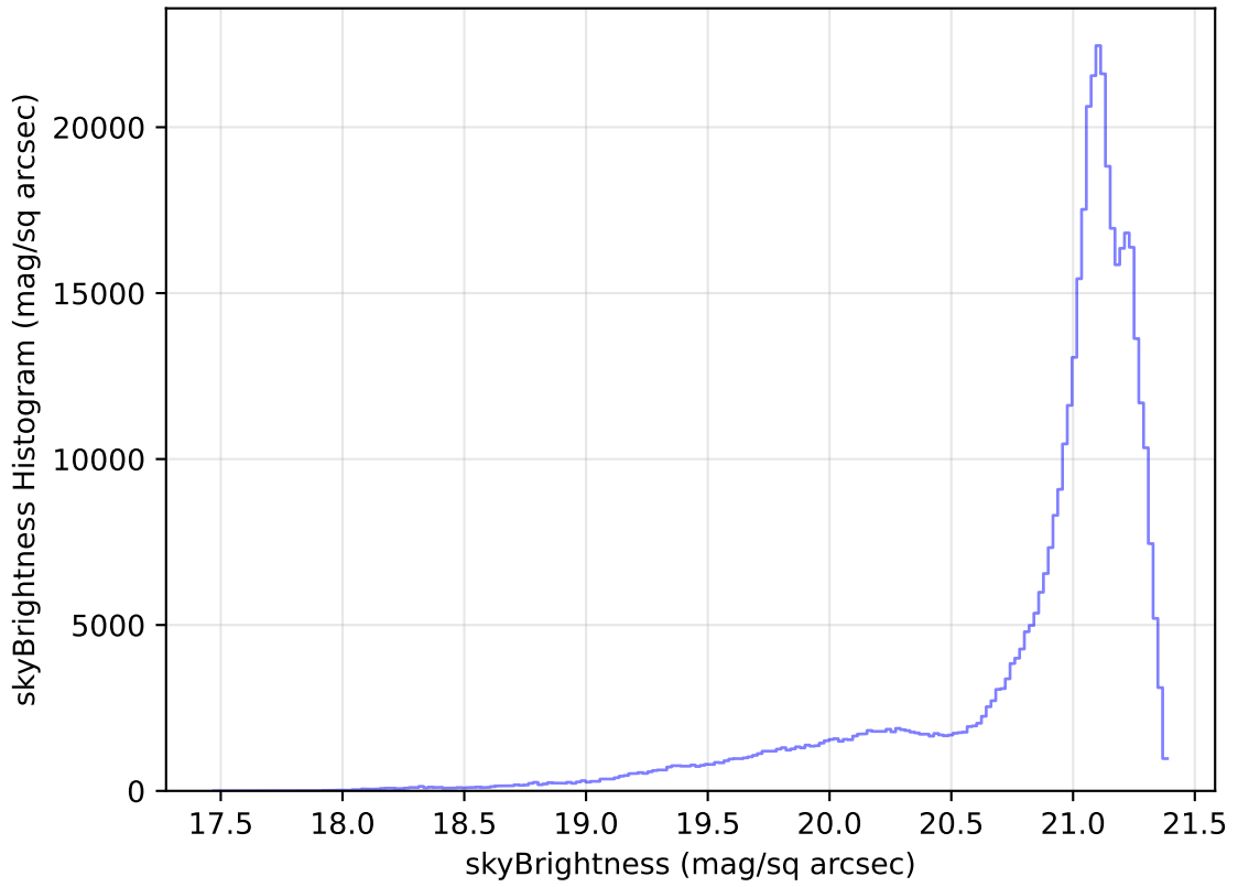
internal_u_expt27_nscale0.9v3.4_10yrs WFD r band: skyBrightness Histogram
