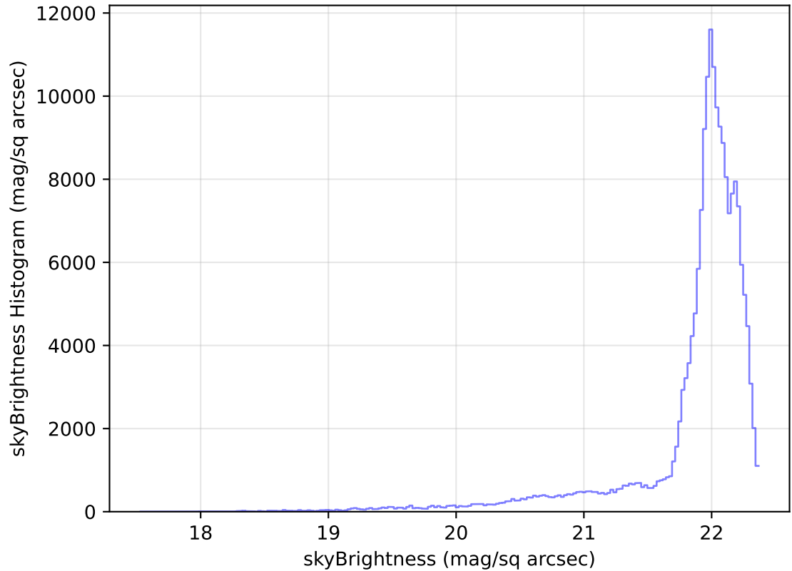
internal_u_expt27_nscale0.9v3.4_10yrs WFD g band: skyBrightness Histogram
