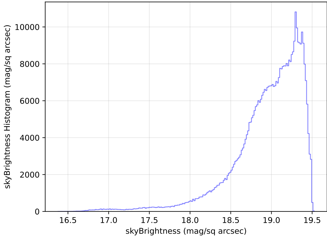
internal_u_expt27_nscale0.9v3.4_10yrs All sky z band: skyBrightness Histogram
