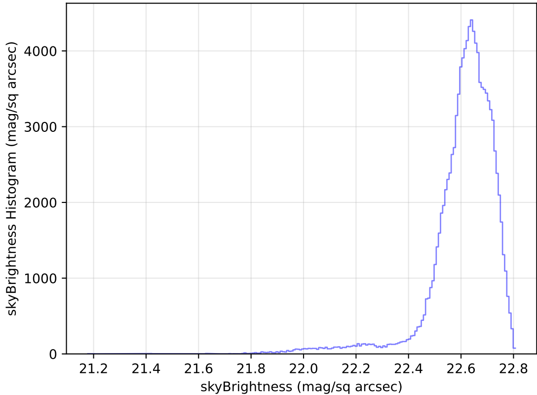
internal_u_expt27_nscale0.9v3.4_10yrs All sky u band: skyBrightness Histogram
