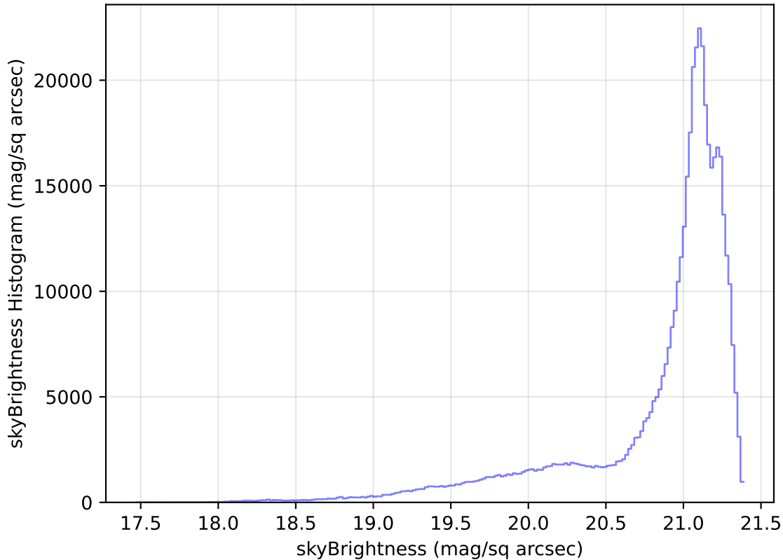
internal_u_expt27_nscale0.9v3.4_10yrs All sky r band: skyBrightness Histogram
