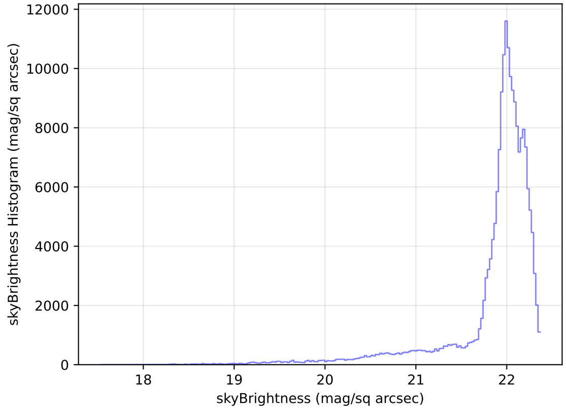
internal_u_expt27_nscale0.9v3.4_10yrs All sky g band: skyBrightness Histogram
