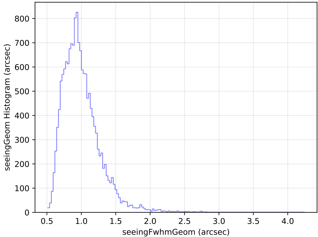
internal_u_expt27_nscale0.9v3.4_10yrs Yr 1 u band: seeingGeom Histogram
