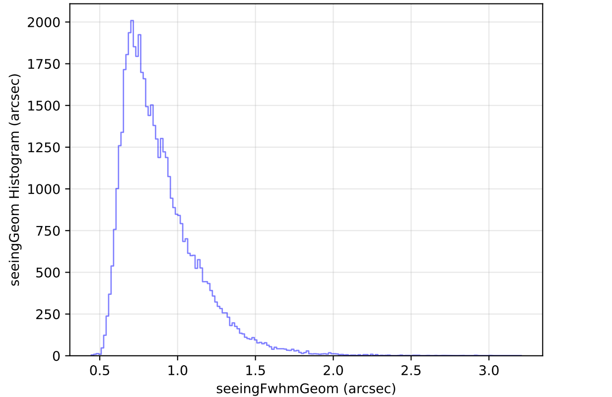
internal_u_expt27_nscale0.9v3.4_10yrs Yr 1 r band: seeingGeom Histogram
